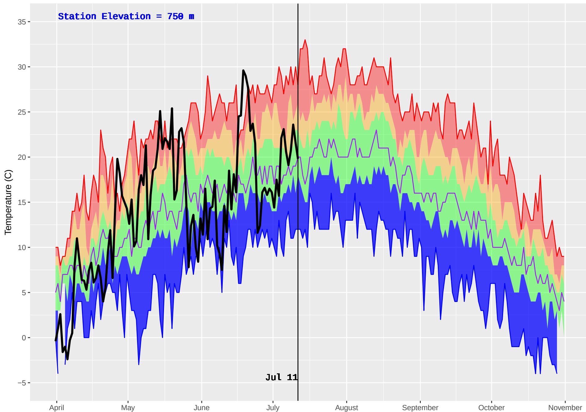
FORT ST JAMES (146) : Historical (1979–2016) and Current (2018) Noon Temperature
