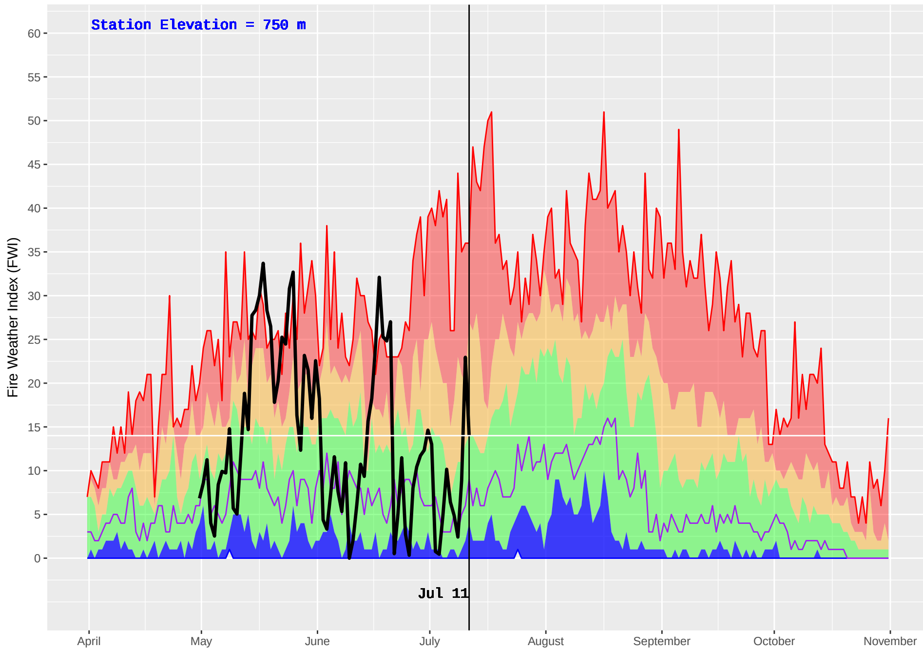
FORT ST JAMES (146) : Historical (1979–2016) and Current (2018) Noon Fire Weather Index (FWI)
