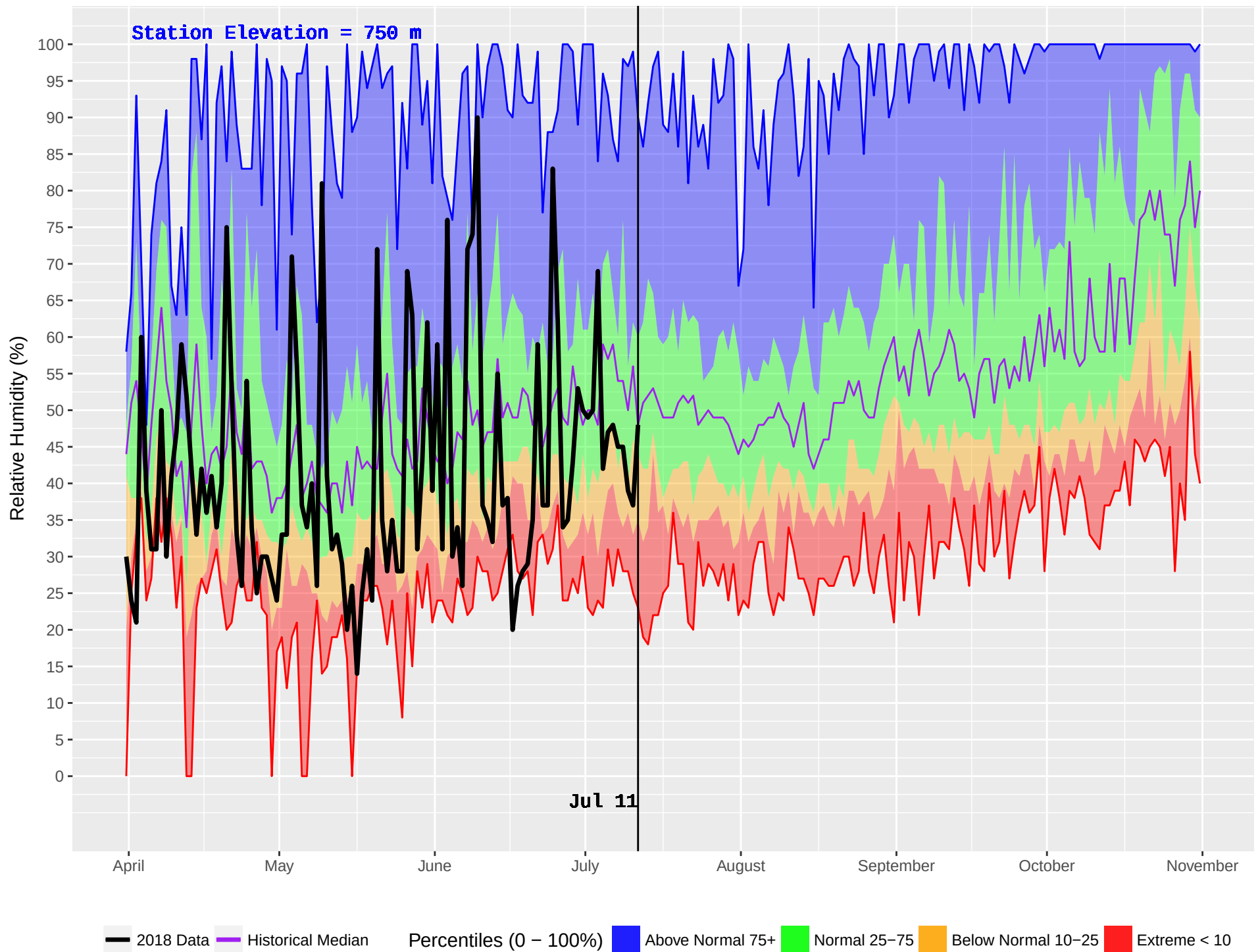
FORT ST JAMES (146) : Historical (1979–2016) and Current (2018) Noon Relative Humidity
