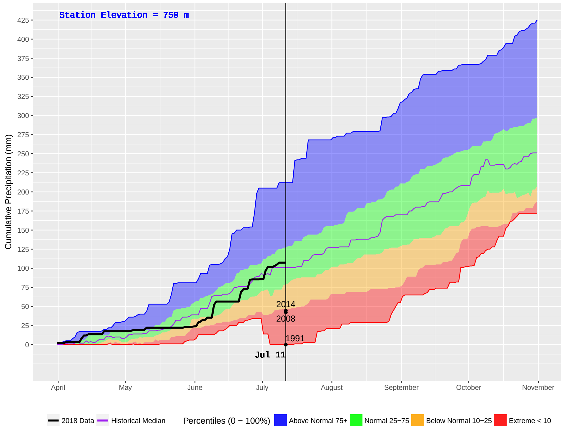
FORT ST JAMES (146) : Historical (1979–2016) and Current (2018) Noon Cumulative Precipitation
