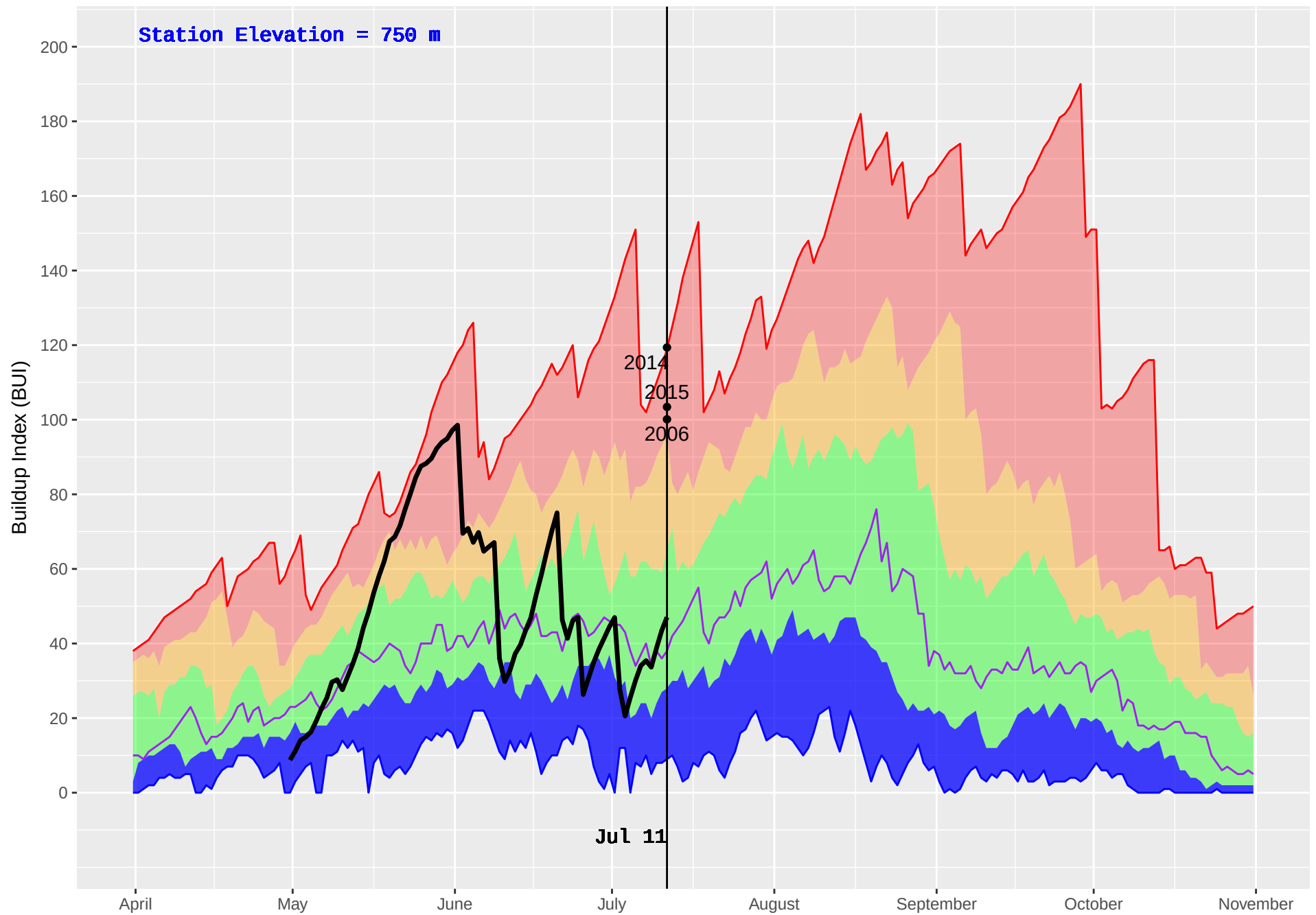
FORT ST JAMES (146) : Historical (1979–2016) and Current (2018) Noon Buildup Index (BUI)
